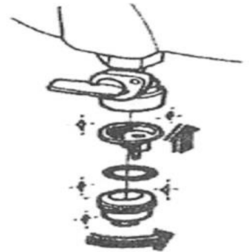
FUEL FILTER ELEMENT ASSEMBLY
